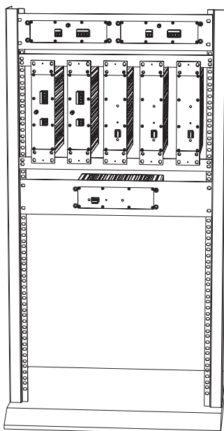
Figure 3. 19"-rack mounting
